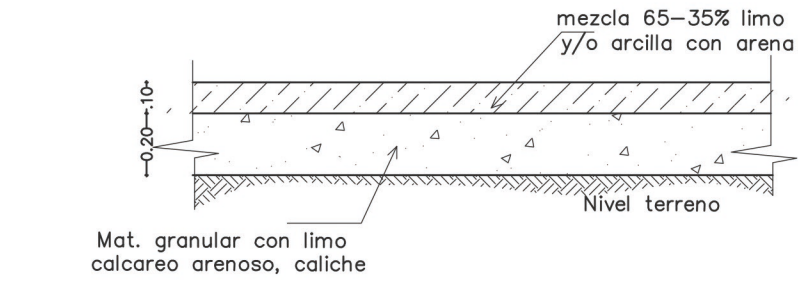
Def. Terreno Media Luna
